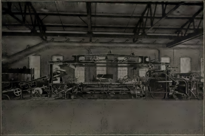
130" HARPER FOURDRINIER PAPER MACHINE.
